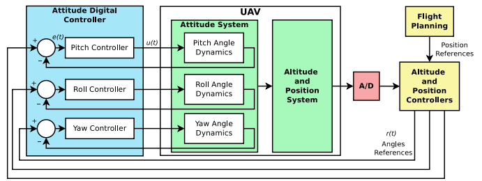
Fig. 10. A typical digital control system for UAVs.
