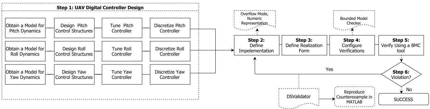
Fig. 6. The proposed methodology for UAV digital-system verification.
