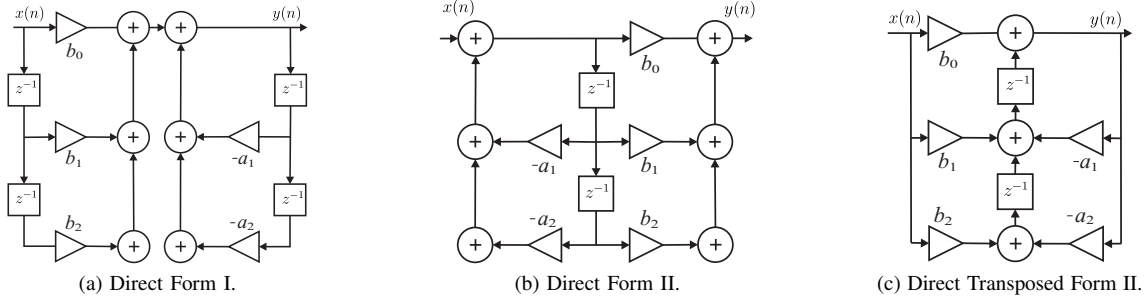
Fig. 3. Direct realizations for digital controllers.
