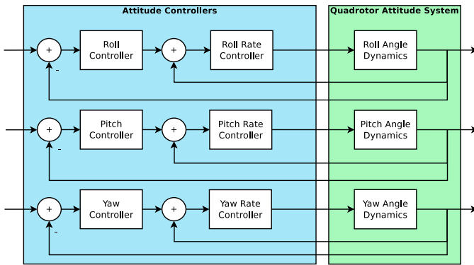
Fig. 11. Attitude control system with combined structure.
