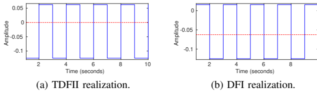
Fig. 17. LCO occurrence in the control torque produced by C_5 , with different realizations and format (13, 3) .
