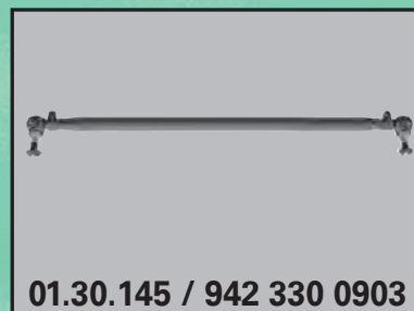
Rod assembly Front axle Length: 1565 mm
