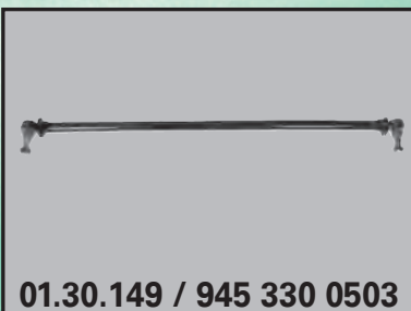
Rod assembly Front axle Length: 1465 mm
