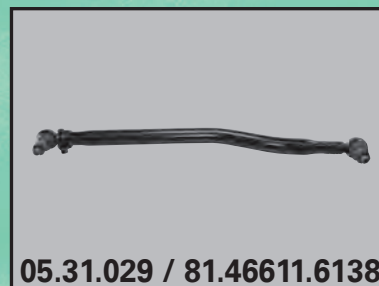
Centre rod assembly Front axle, push rod
