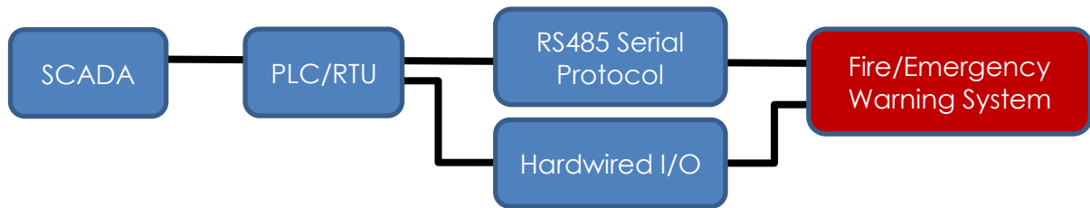
Figure 4-1 – Control System Boundaries
