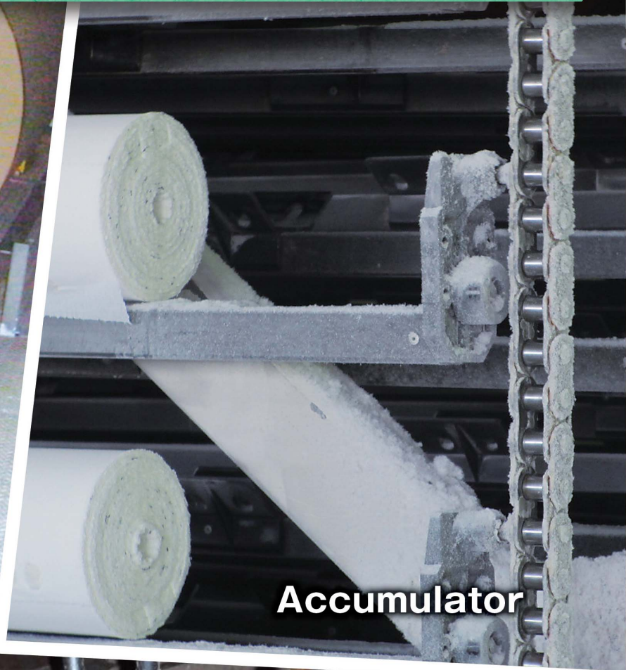
Web Conveyance
