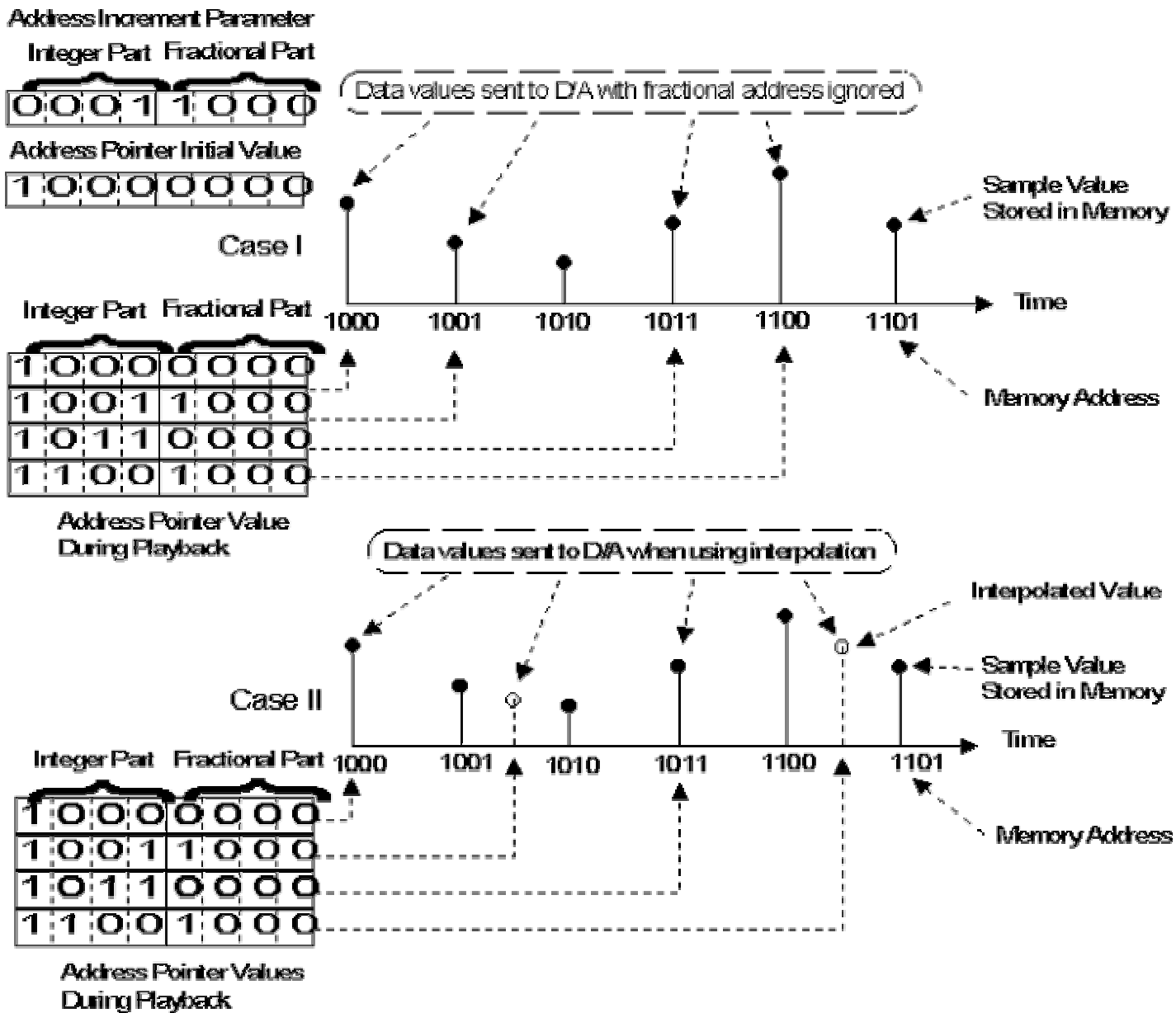
Figure 8: Sample Memory Addressing and Interpolation
