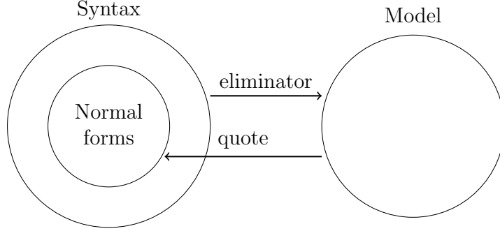
Figure 5.1: Normalisation by evaluation
