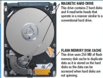
FIGURE 3-8 Hybrid hard drives contain both magnetic hard disks and a large quantity of flash memory for increased performance.
