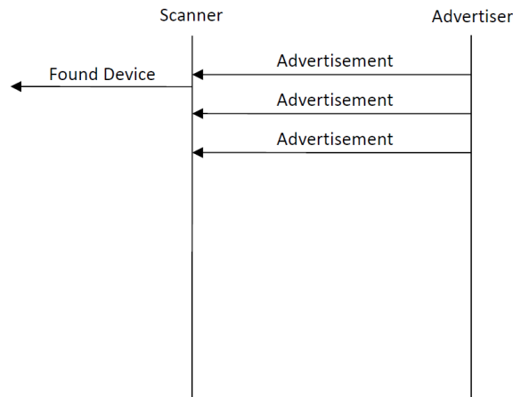
Figure 4.2. Passive Scanning
