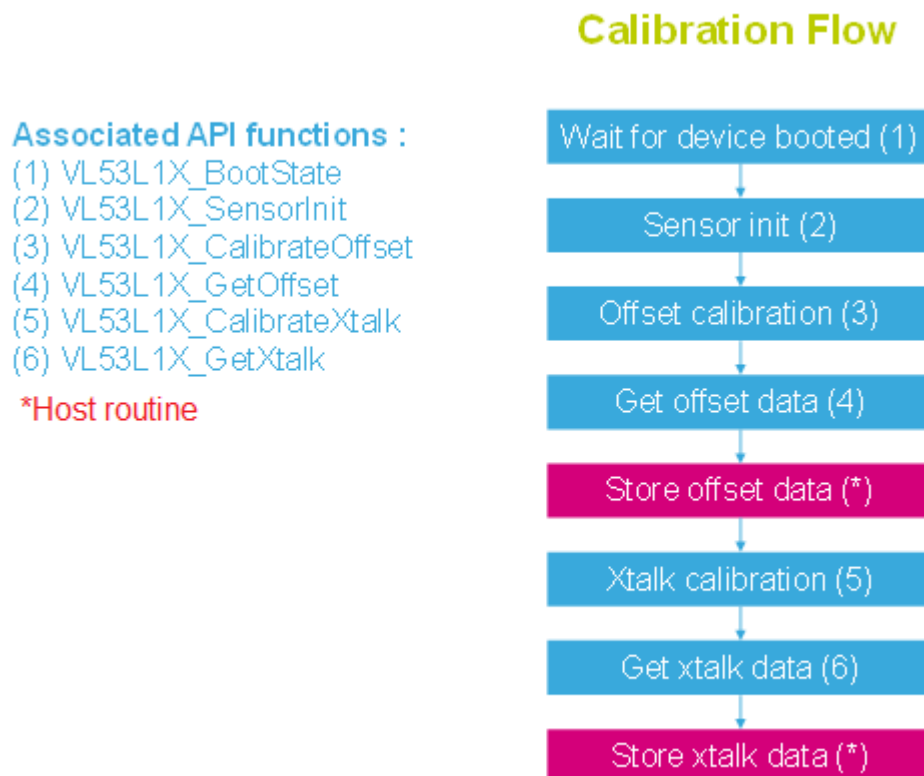
Figure 4. Calibration flow
