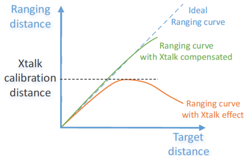
Figure 6. VL53L1X crosstalk calibration distance definition
