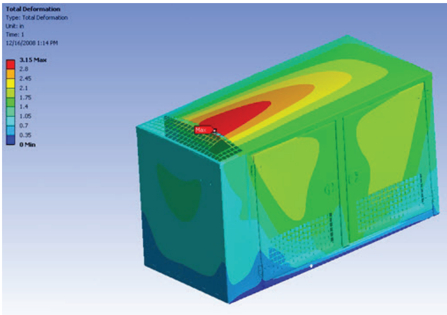
Figure 3: Analytical Deflection Plot Due to Basic Wind Speed Load on Enclosure Source: Kohler Power Systems
