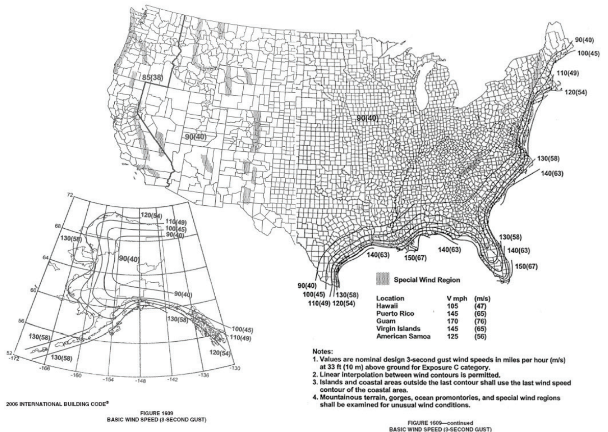
Figure 1: IBC Basic Wind Speeds
