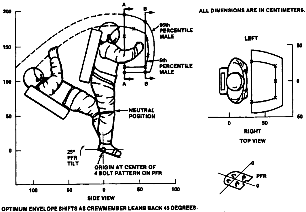
Figure 3. Reach envelopes for EMU operations while in the portable foot restraint.
