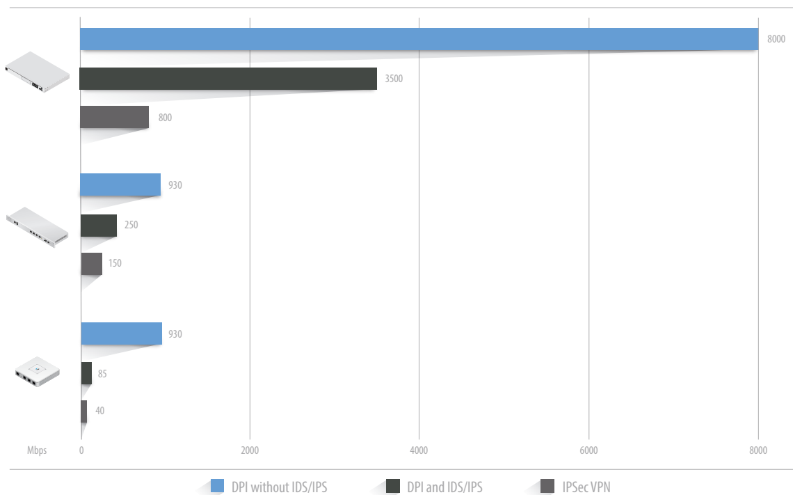
Downlink Throughput
