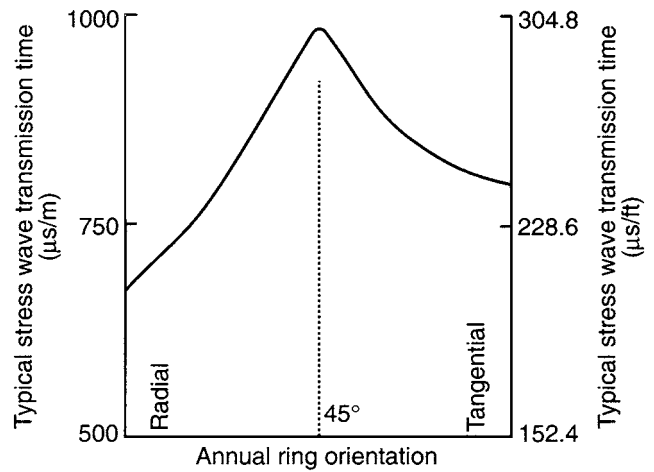
Figure 3.4—Transverse stress wave transmission time compared with annual ring orientation.
