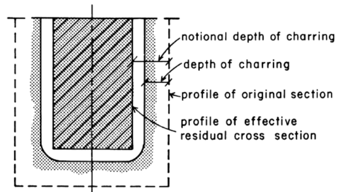
Figure 5.5—Residual cross section of a charred wood member.
