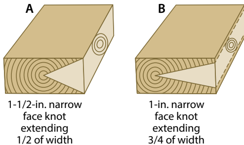
Figure 6.5—Diagram from a pocket guide showing measurement of knots on 2- to 4-in. lumber that included structural joists and planks (SPIB 2002). Used courtesy of Southern Pine Inspection Bureau.
