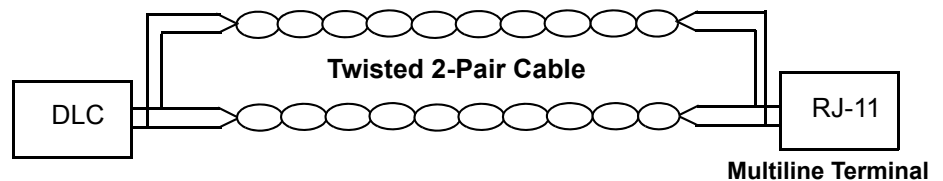
Figure 5-4 Connecting the DLC Using Twisted 2-Pair Cable
