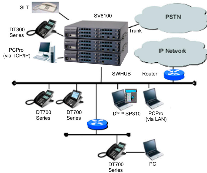
Figure 1-6 Simplified SV8100 System (19") Connectivity
