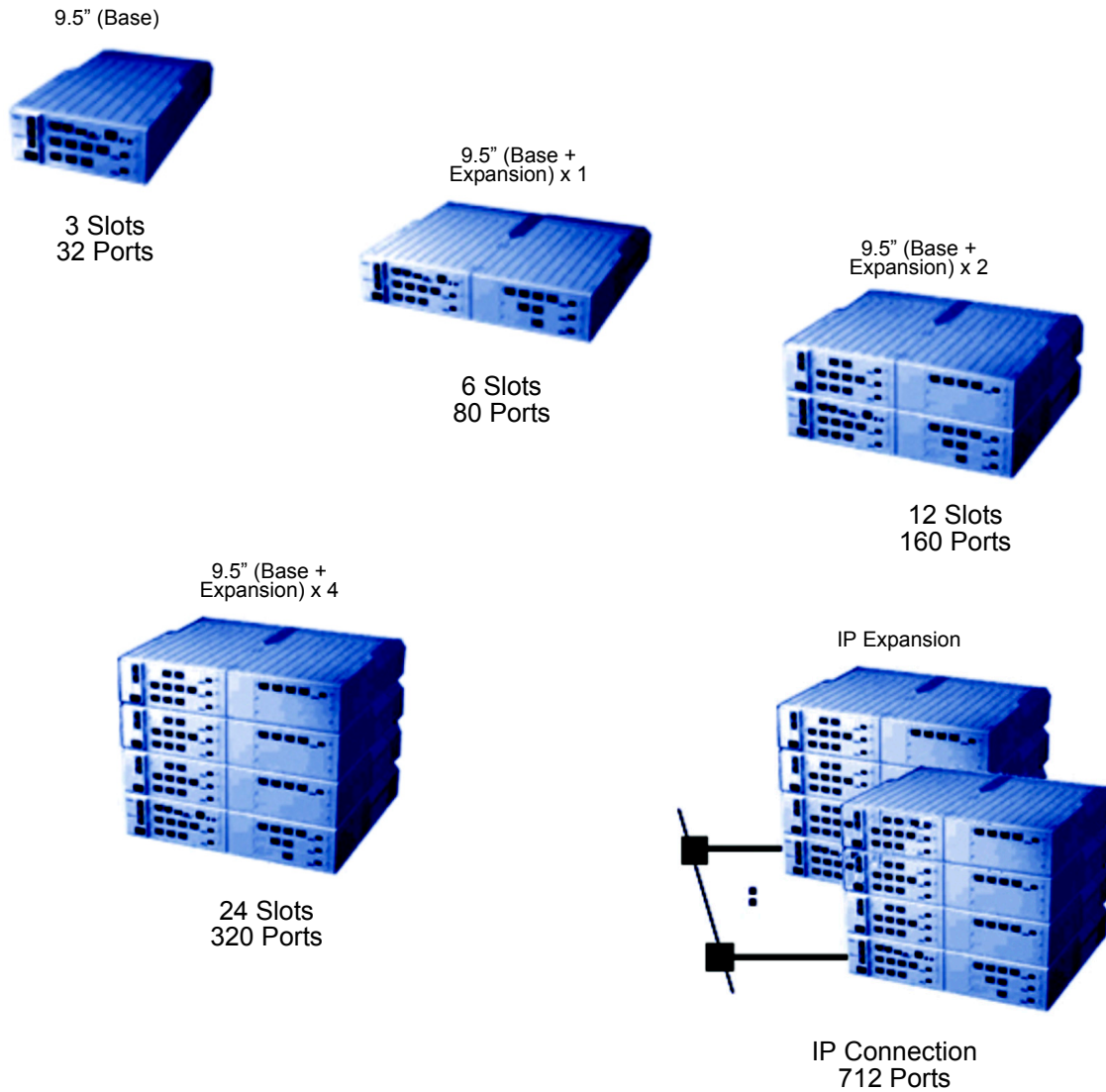
Figure 5-3 CHS2U B-US Base and CHS2U E Expansion Chassis
