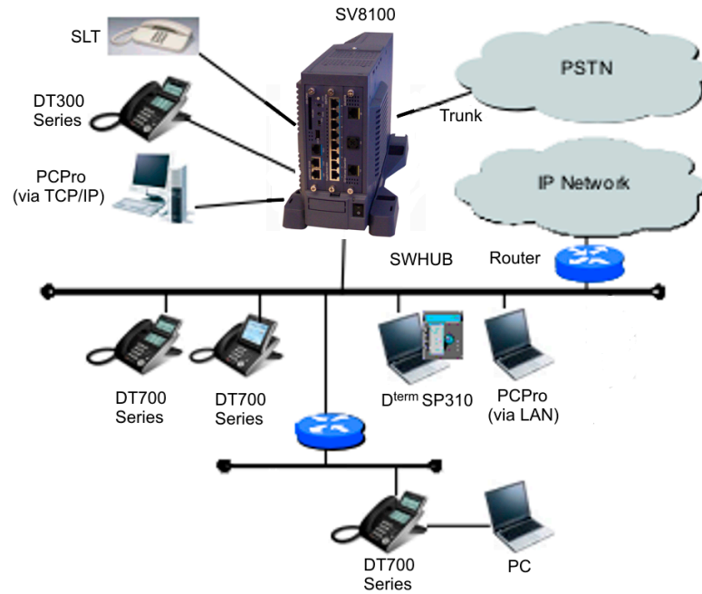
Figure 1-5 Simplified SV8100 System (9.5" Gateway and Base) Connectivity
