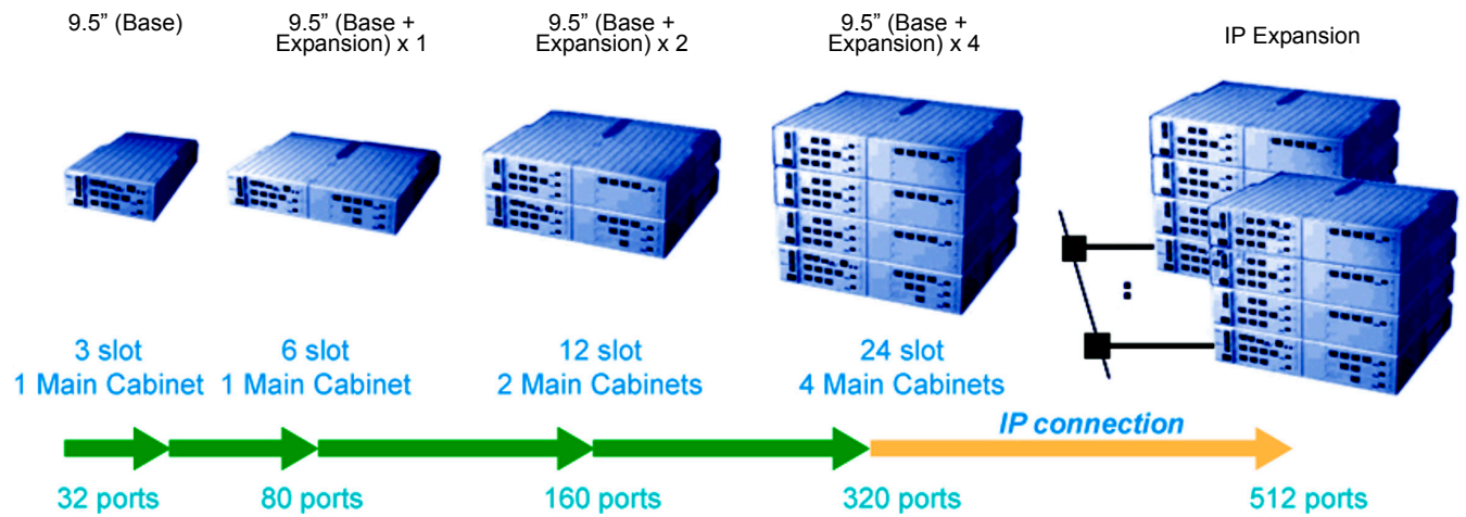
Figure 1-3 UNIVERGE SV8100 CHS2U B-US and CHS2U E Chassis Expandability
