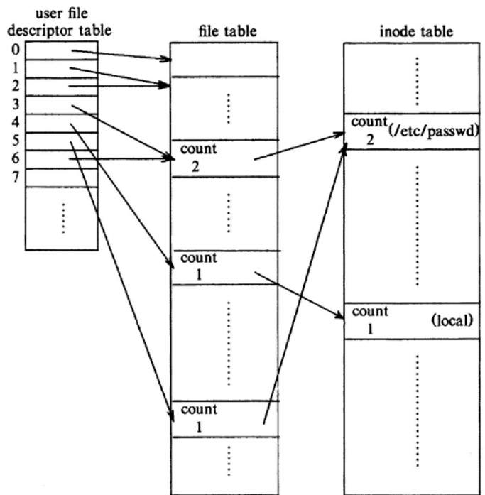
Data structures after dup
