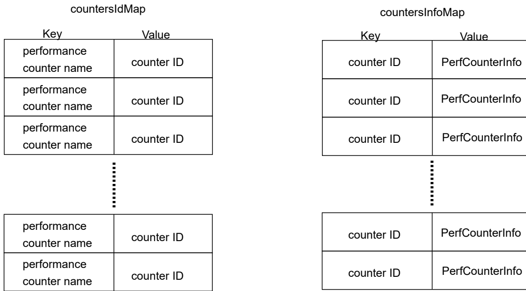
Figure 17-2. Performance Counter Hash Maps
