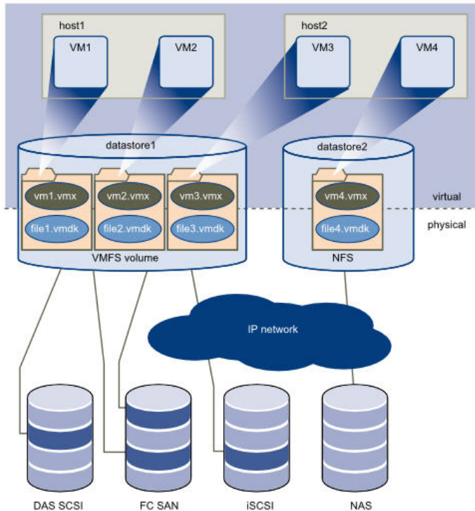
Figure 8-1. Storage Architecture
