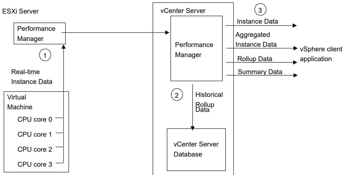
Figure 17-1. vSphere Performance Data Collection and Retrieval
