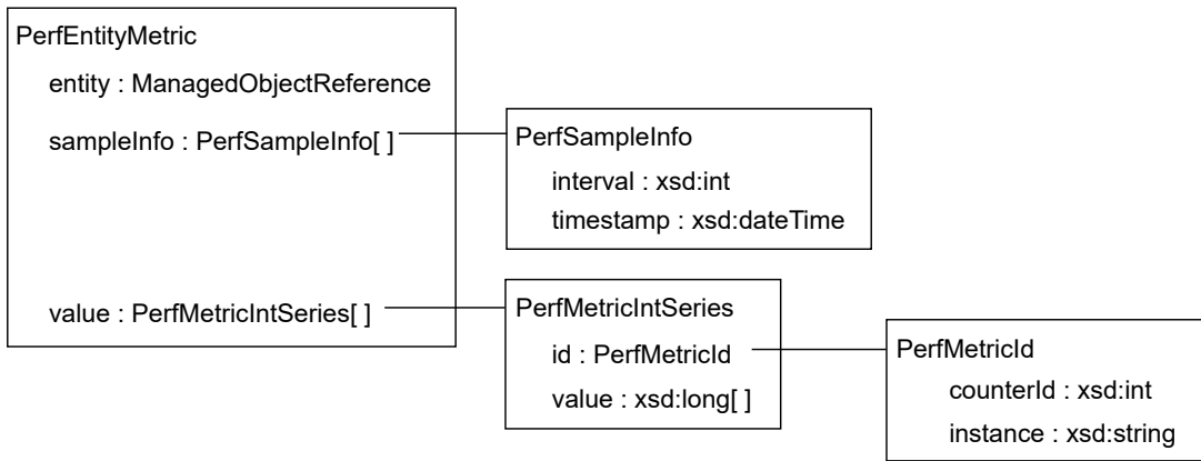
Figure 17-3. PerfEntityMetric Object Hierarchy
