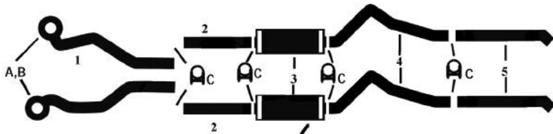
Typical muffler location for Extreme mufflers
