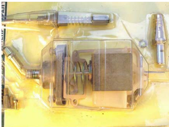
K65/K63T Carburetor Repair Set Part #: 1107500 Vendor Part #: 000.377 List Price: 22.18€ ( www.oldtimergarage.eu )
