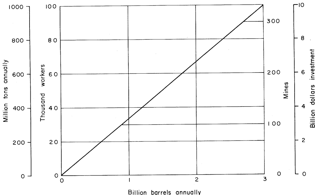
Figure 7 - Mining requirements for production of specified quantities of motor vehicle fuel from coal. Tonnage is based on conversion rate of 3 barrels of gasoline per ton of coal.
