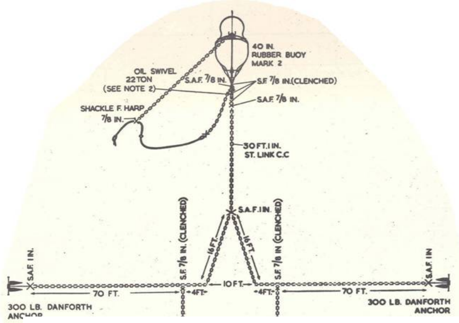
Figure 17: Schematic of British anti-snatch system
