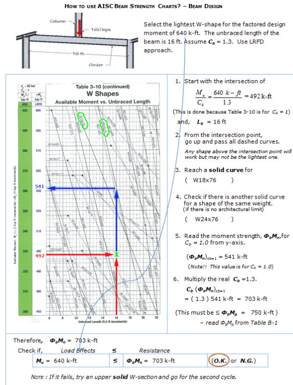
Figure 6 AISC Beam Design Process visualized
