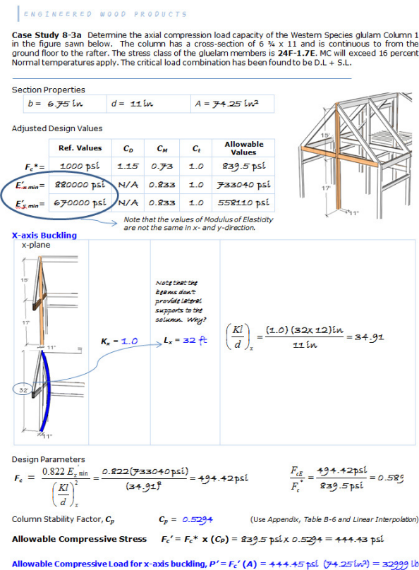
Figure 3 Column Strength including Buckling
