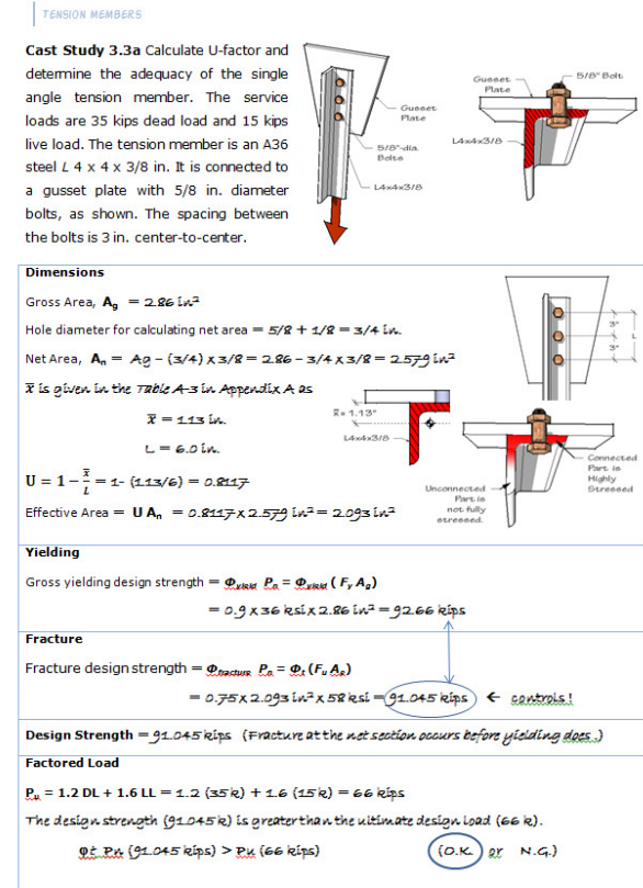
Figure 5 Tension Member Design with Shear Lag visualized
