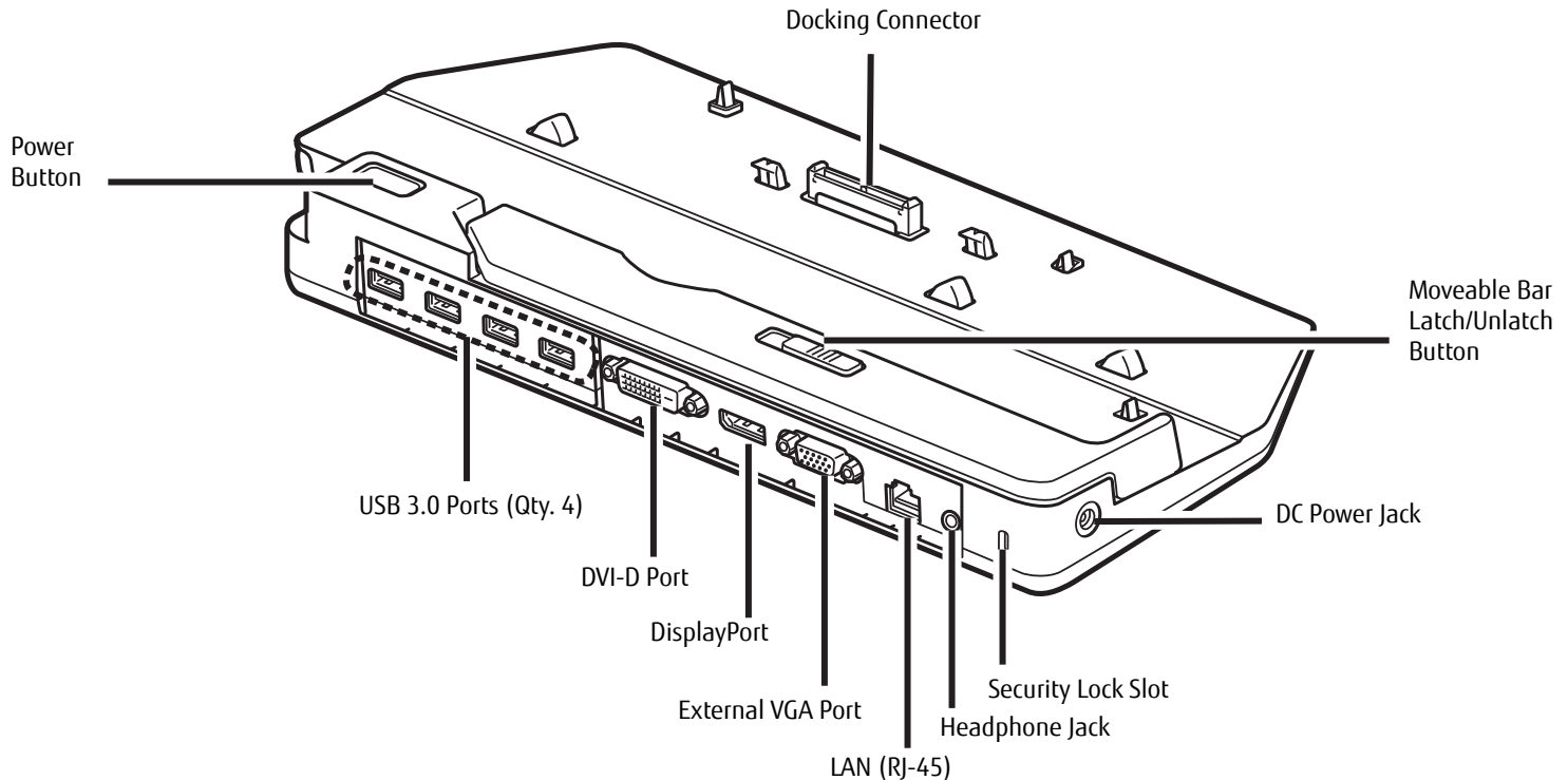
Figure 43. Port Replicator - Rear
