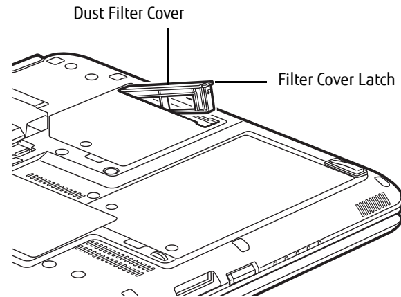
Figure 48. Removing the Dust Filter Cover
