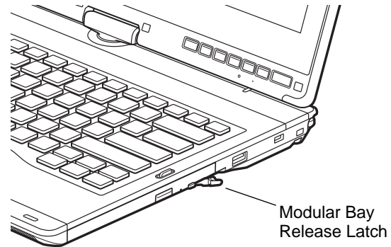
Figure 29. Removing/Installing Modular Device
