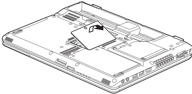
Figure 36. Opening Memory Compartment
