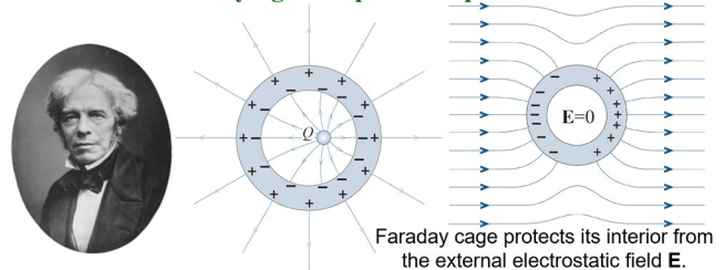
Fig. 3. Example 3 of Conceptual Questions in Electromagnetics [20] dealing with electrostatic shielding, along with an outline of a common misconception and underlying concepts and equations. The correct answer is (B). Figures from [21].
