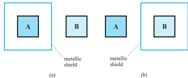
Figure 1.27 Two proposed configurations for electrostatic shielding; for Conceptual Question 1.31.
