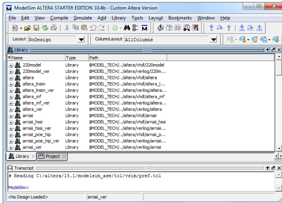
Figure 7. ModelSim window.
