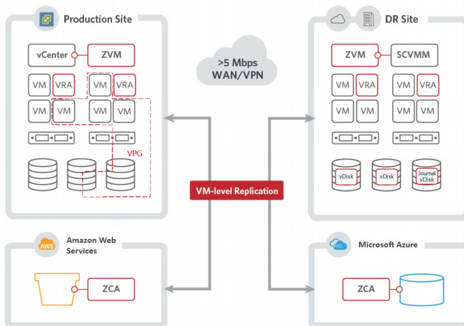
Figure 2. Zerto Architecture
