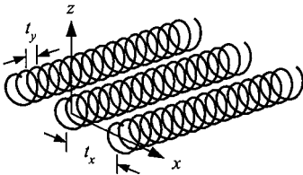
Figure 1 Geometry of chiral sail.
