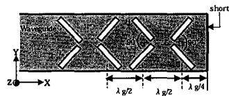
Fig.1: Array configuration
