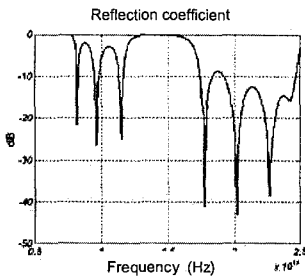
Figure 1.a Reflection coefficient according to frequency
