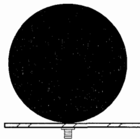
Fig 1 Wideband circular disk monopole antenna solution first reported by Honda et al.
