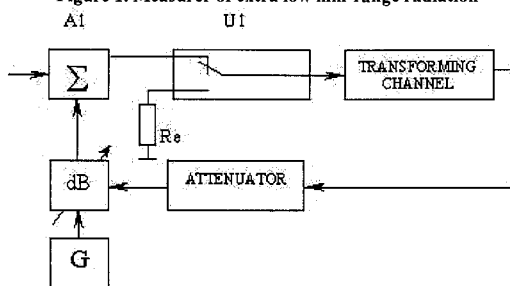
Figure 1. Measurer of extra low mm-range radiation
