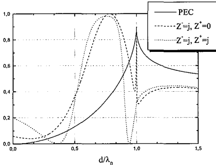
Fig.2. Frequency dependence of the reflected powers. 2w/d=0.5 , \varphi=0^0
