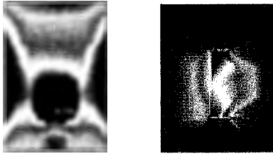
Fig.2: Current distribution showing the antenna isolation, - on the left, for a PIFA with very low isolation and a lot of current on the edges. - on the right, for an Ethertronics antenna with very little current on the edges.
