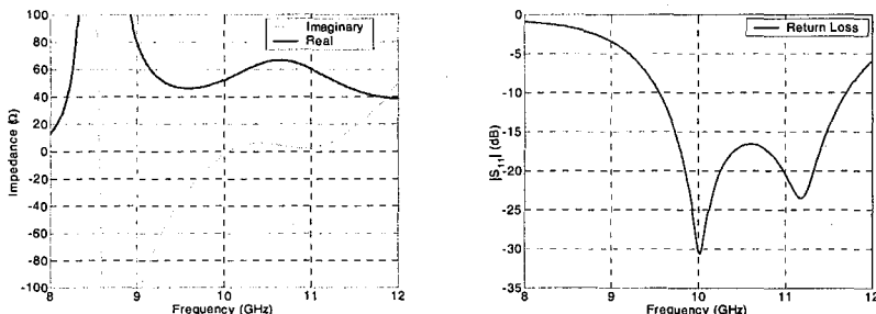
Fig. 2. Input impedance and return loss.
