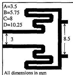
Fig. 1. Antenna geometry.
