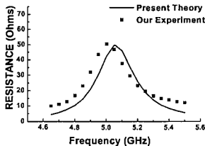
Fig. 2. Input Resistance vs. Frequency
