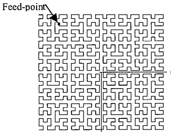
A fifth step Hilbert-curve Antenna
