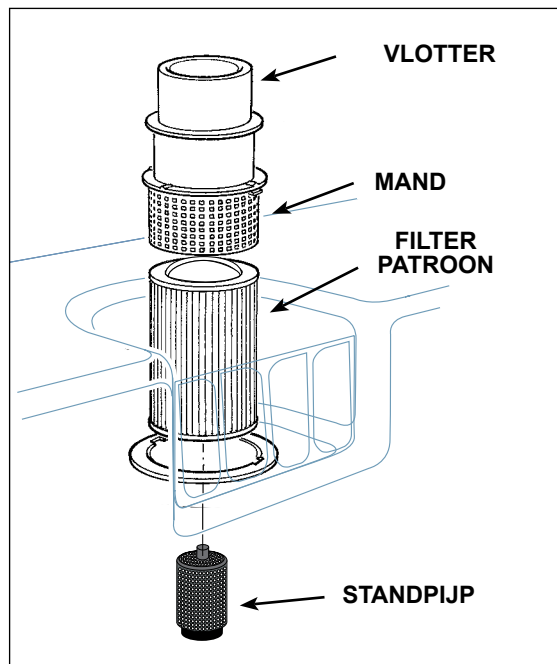
FILTERSISTEEM
