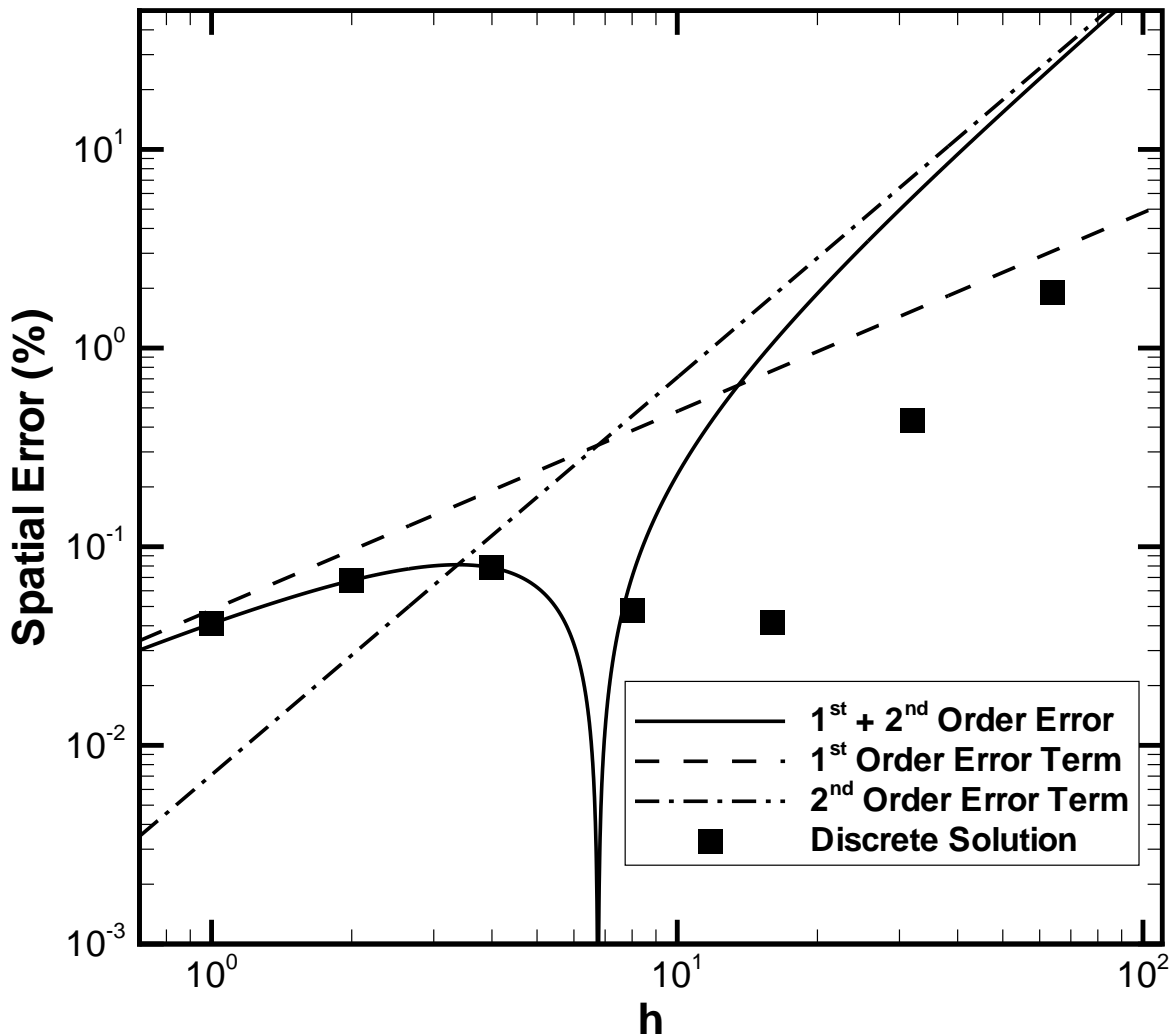
Figure 5. Demonstration of extrapolated error estimation for mixed first and second order schemes [286].
