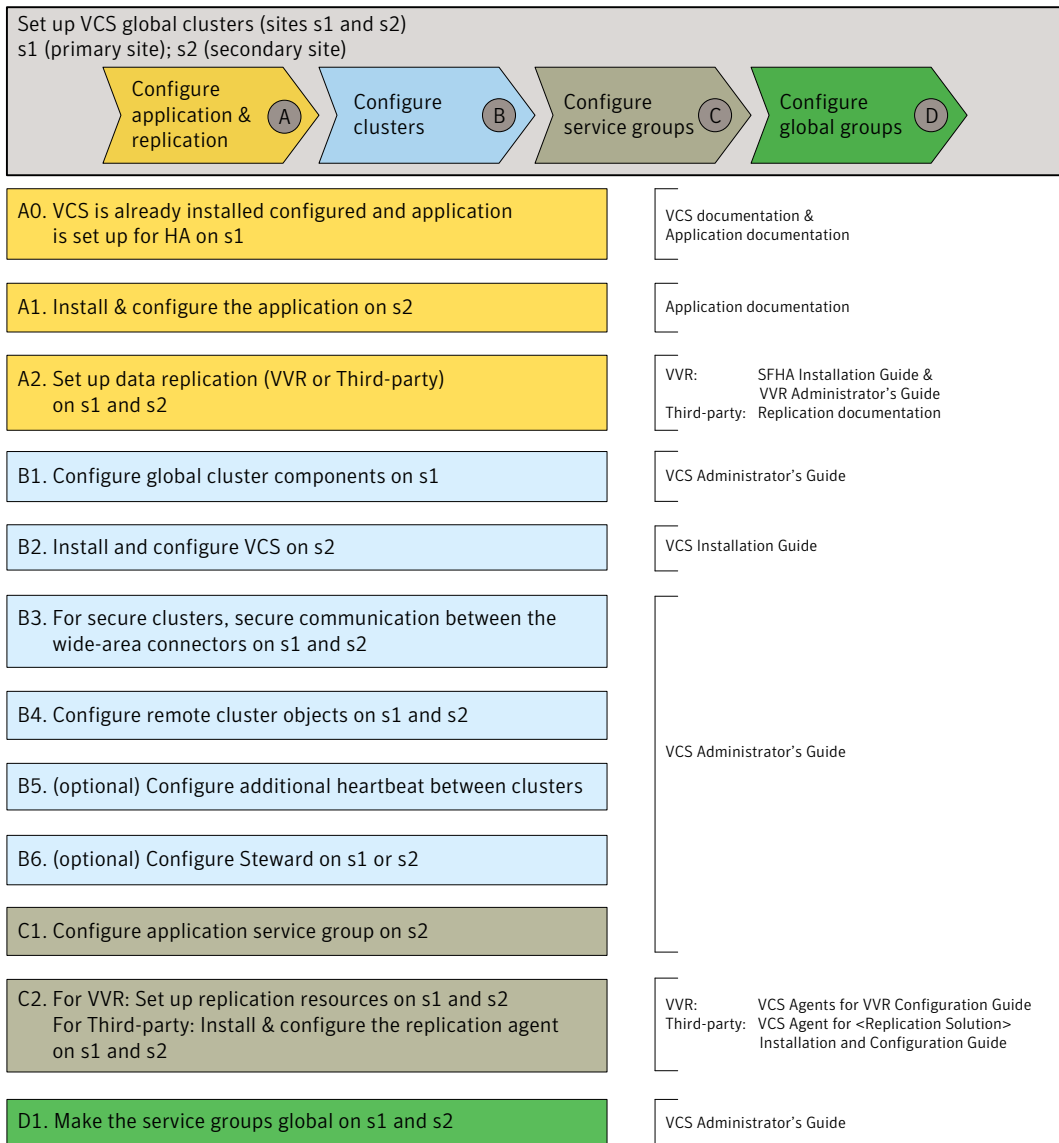
Figure 16-4 High-level workflow to set up VCS global clusters
