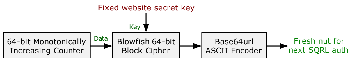
Figure 19: Algorithmic Nut Synthesis
