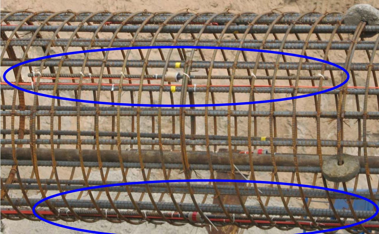
A pile cage with an array of 4 Sister
