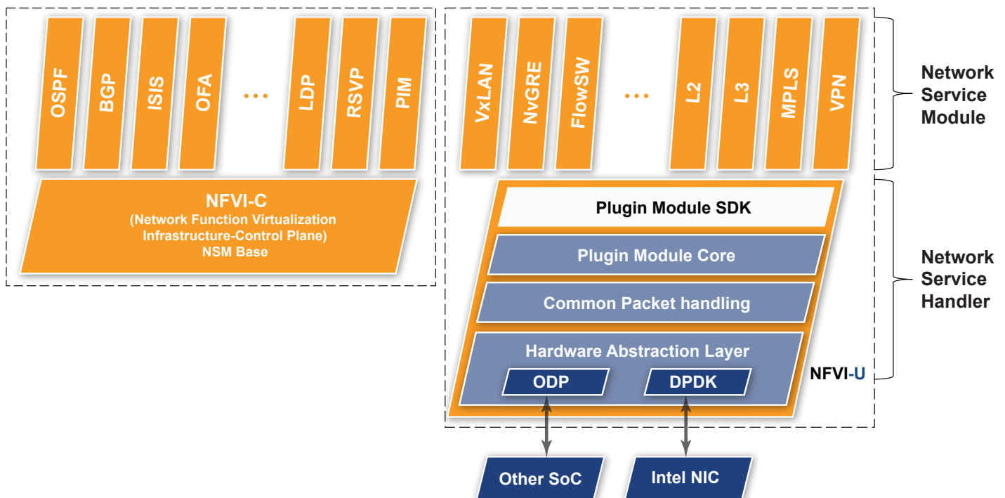
Figure 3. VirNOS: Data Plane Infrastructure
