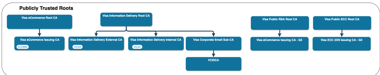
Figure 1–1: PKI Hierarchies
