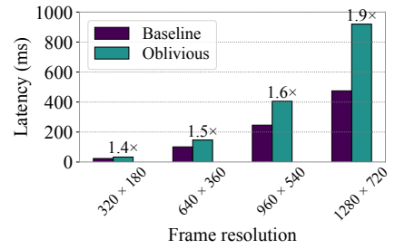
Figure 15: Oblivious object tracking.
