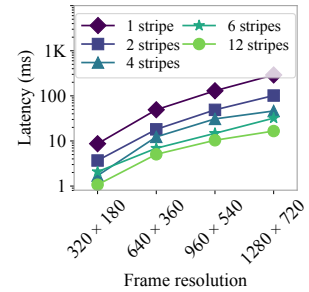
Figure 12: Latency of oblivious bounding box detection.
