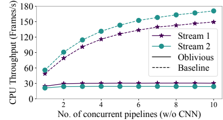
Figure 18: CPU throughput (pipeline 1).
