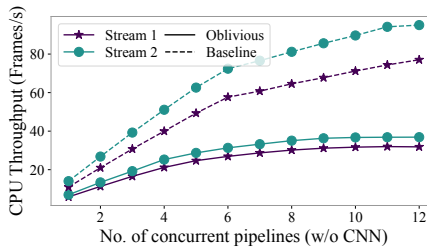
Figure 19: CPU throughput (pipeline 2).
