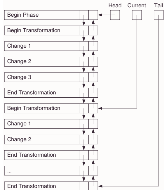
Figure 12: Data structure used for undoing transformations.
