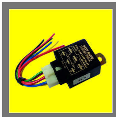
Headlamp Relay with 6" Wiring (24 Volts)
