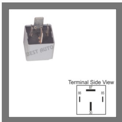
Heavy Duty Relay 12V / 24V 4 Pin
