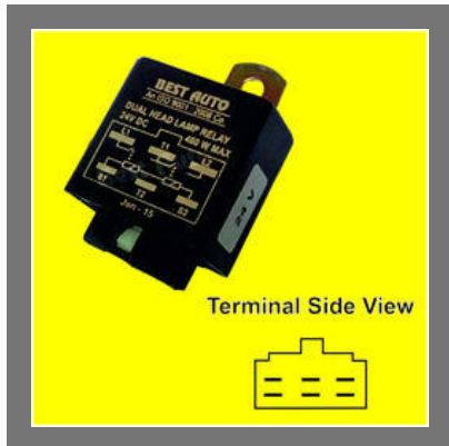
Headlamp Relay (24 Volt) - X8003800 / 911125
