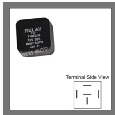
Telco Relay 5 Pin 12V / 24V Plastic Body - 2654-5420-4913, 2608-5450-4901
