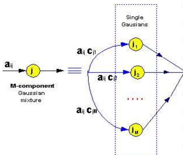
Fig. 4.4 Baum-Welch algorithm
