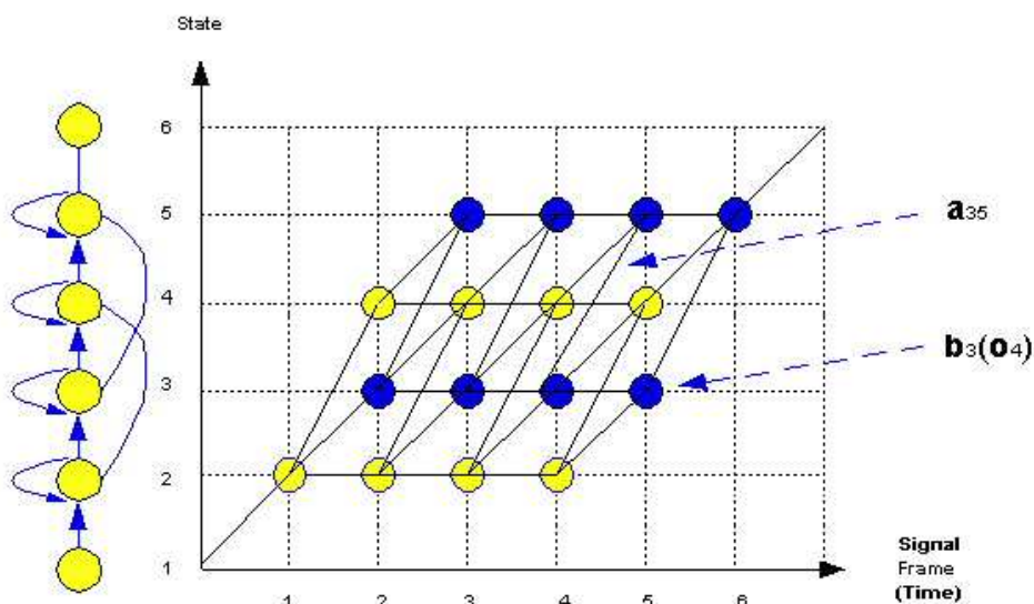
Fig. 4.3 Viterbi algorithm
