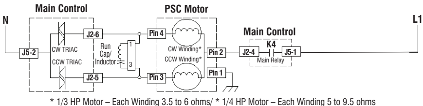
Figure 5 - PSC Motor Strip Circuit (shown in ON position)
