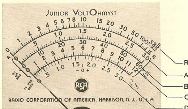
Figure 3. Details of WV-77C scales
