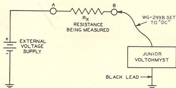
Figure 2. Circuit for measurement of resistance values above 1000 megohms.
