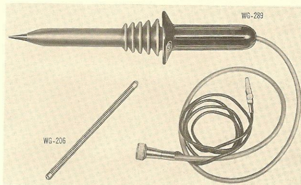
Figure 4. Accessory high-voltage probe and multiplier resistor for use with the WV-77C
