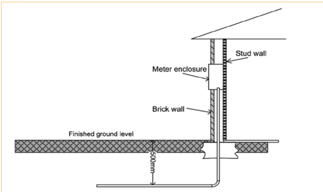
Figure 9.4(b) Conduit entry through slab – brick veneer
