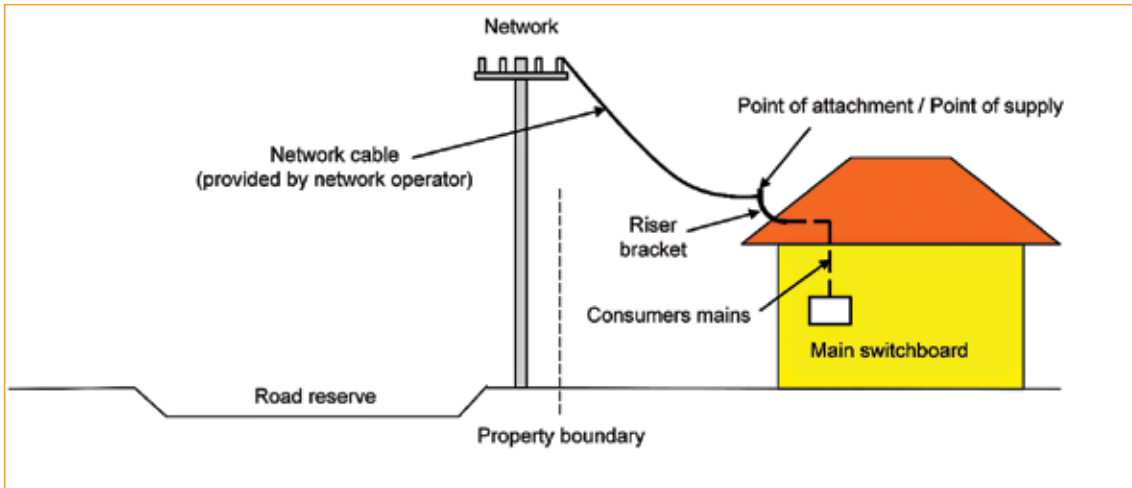
Figure 3.1 Overhead service
