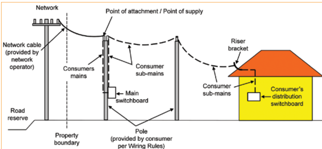
Figure 3.4 Overhead supply to rural consumer 2
