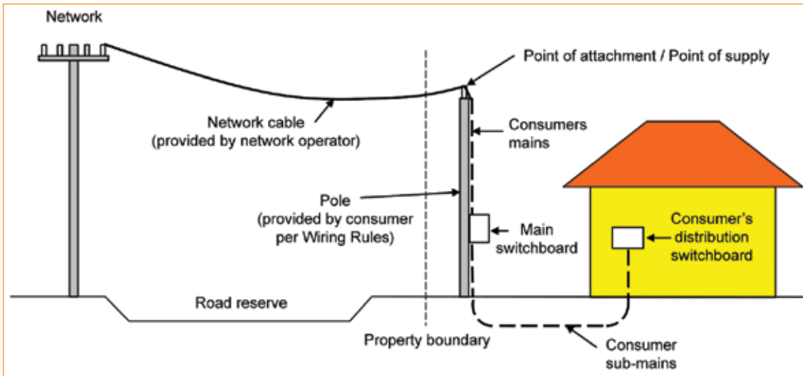
Figure 3.3 Overhead supply to consumer's pole/main switchboard
