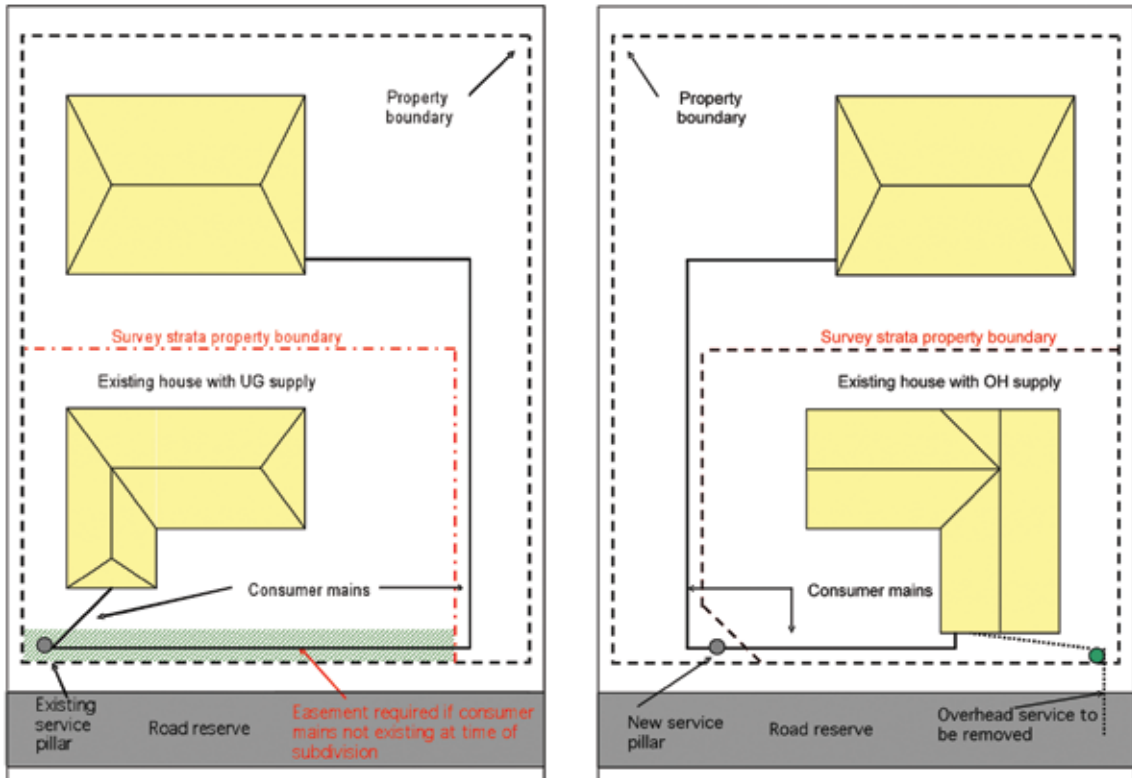
Figures 3.8(e) & (f) Examples of ‘battle-axe’ subdivision with and without easements 3
