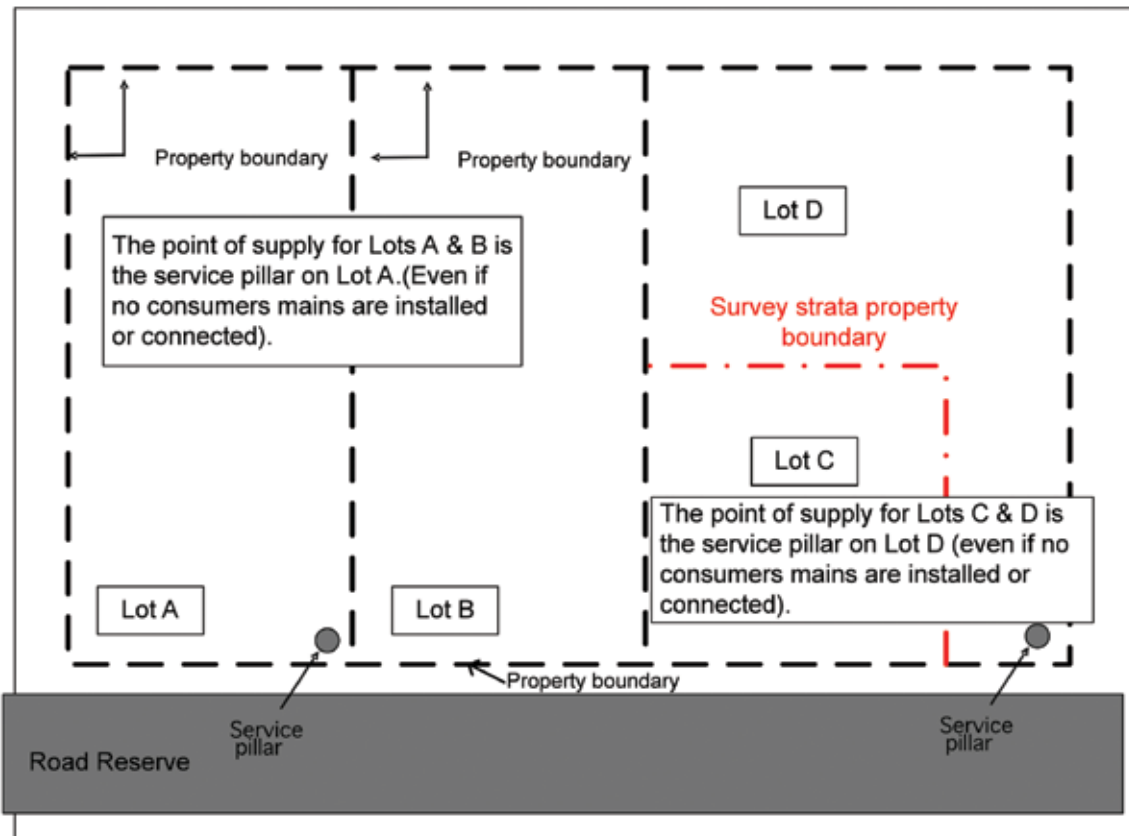
Figure 3.8(a) Example of points of supply
