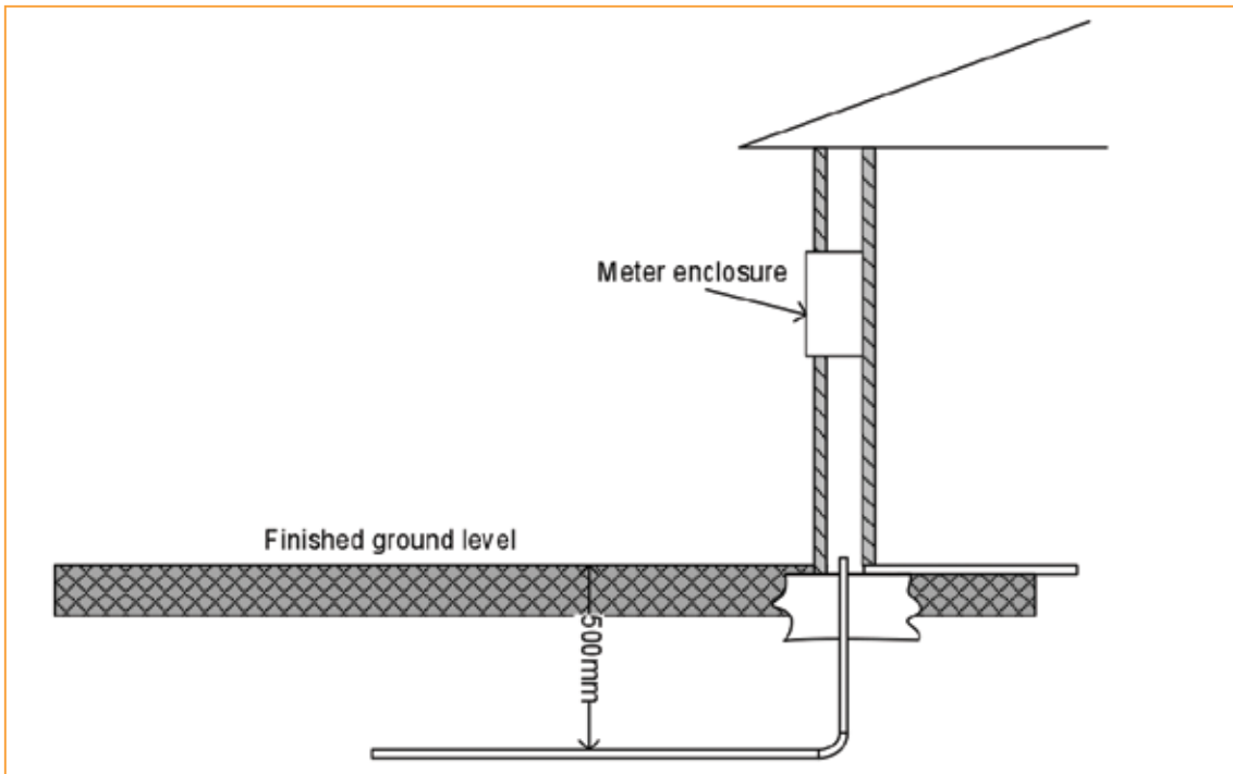
Figure 9.4(a) Conduit entry through slab – double brick
