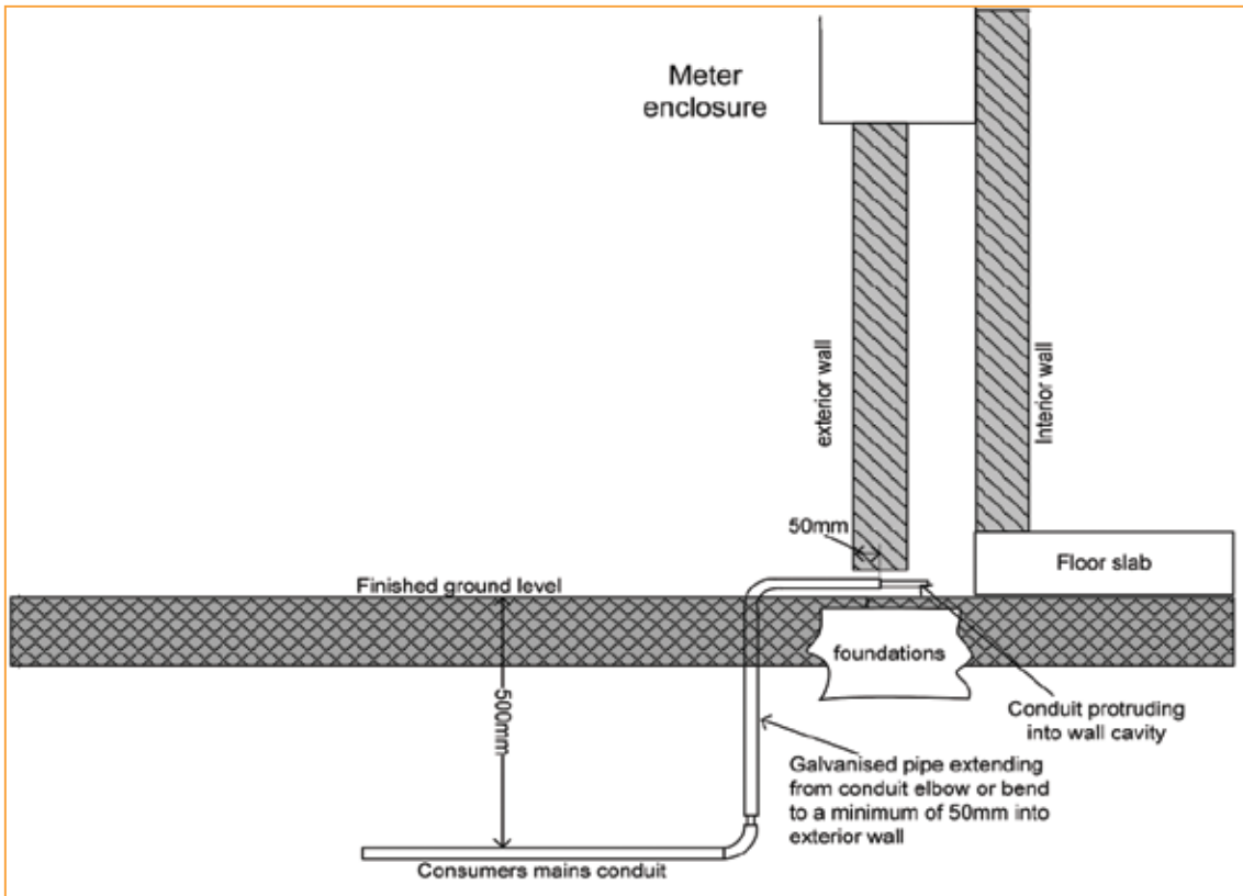
Figure 9.4(c) Conduit entry through wall – double brick
