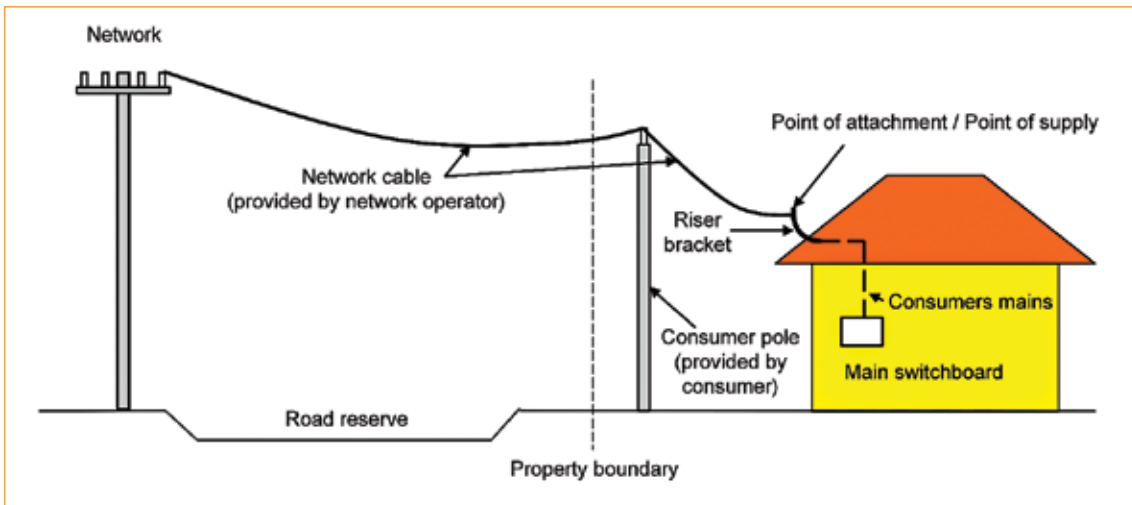
Figure 3.2 Overhead service with consumer pole
