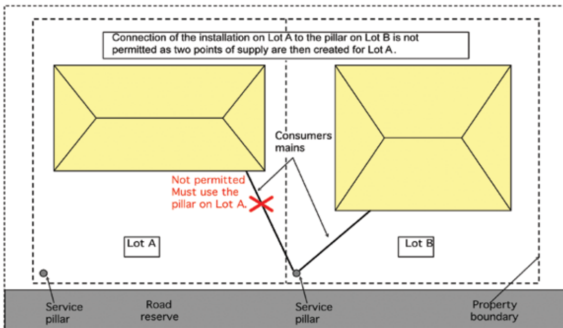
Figure 3.8(b) Example of points of supply
