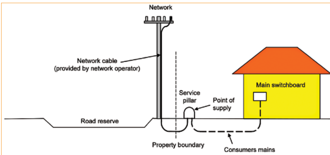
Figure 3.5 Overhead street mains and underground consumers mains
