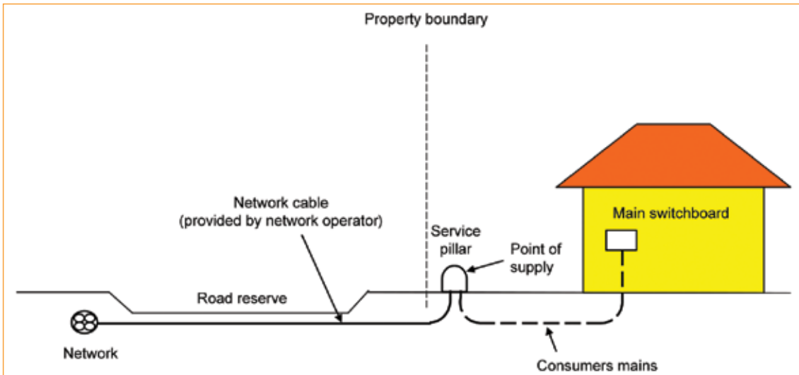
Figure 3.6 Underground network and underground consumers mains
