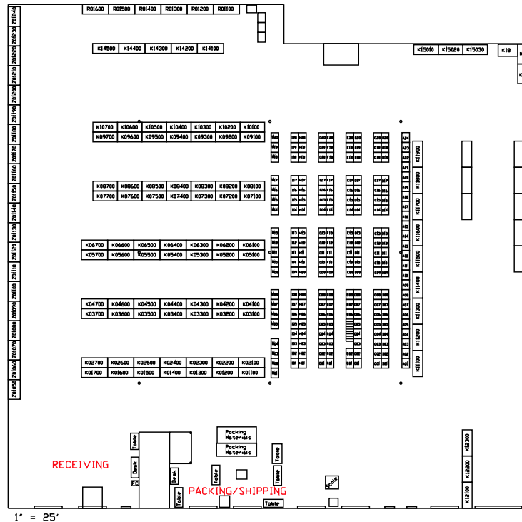
Figure 6.12: Question 6.8: Critique this layout of a service parts distribution center.
