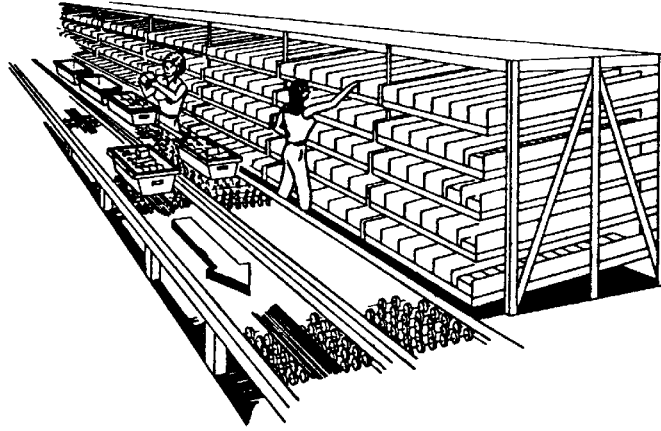
Figure 5.3: Gravity flow rack for cartons. (Adapted from “Warehouse Modernization and Layout Planning Guide”, Department of the Navy, Naval Supply Systems Command, NAVSUP Publication 529, March 1985, p 8-17.)
