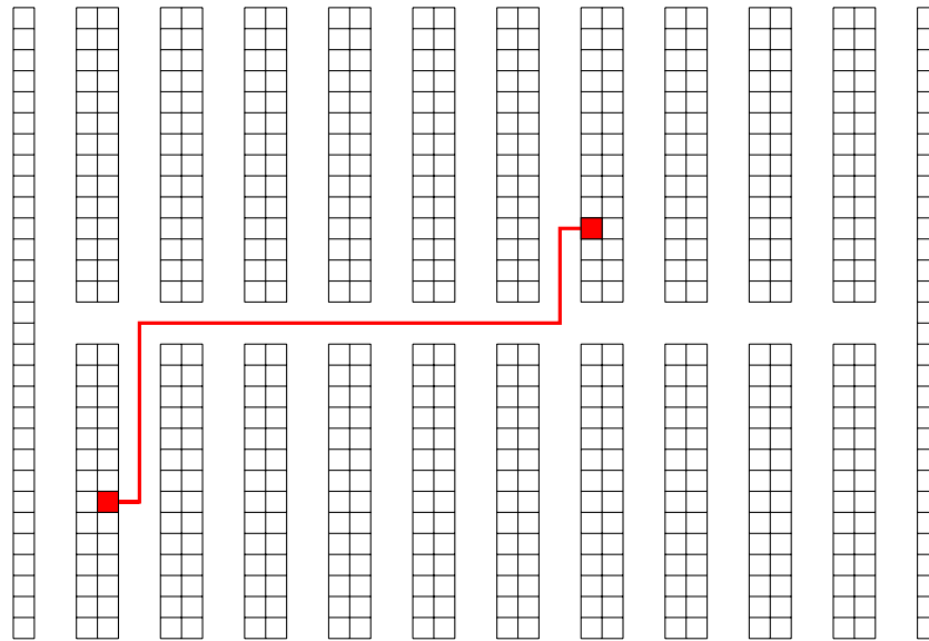
Figure 6.5: A cross-aisle allows more direct and therefore shorter travel between storage locations.
