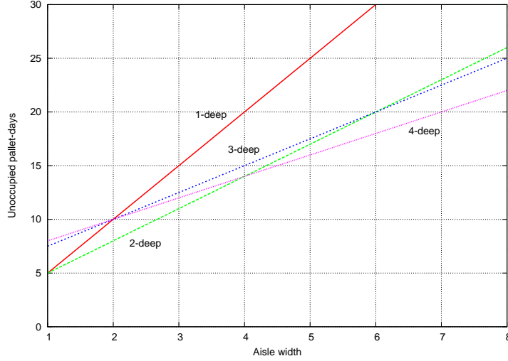
Figure 6.9: Waste, measured as pallet position-days that are unoccupied but unavailable, depends on both the lane depth and the aisle width. The four pallets of this sku should be stored either 2-deep or else 4-deep, depending on the width of the aisle.
