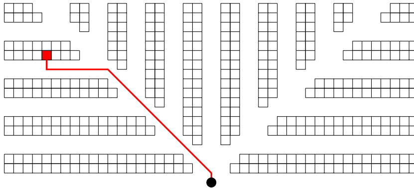
Figure 6.6: Angled aisles, suggested by Gue and Meller, allow more direct travel between storage and a central location of receiving/shipping (at the bottom).
