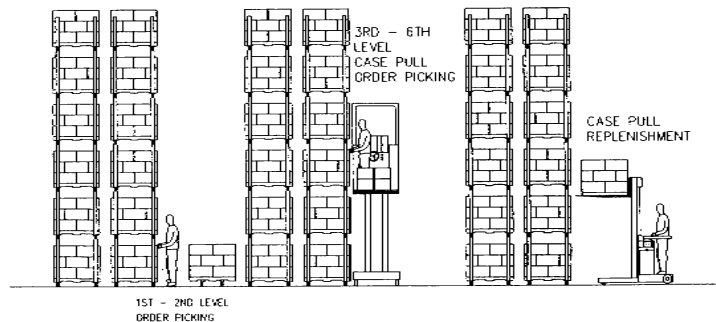
Figure 7.2: Cartons are picked from the bottom, most convenient, level; when the bottom position has been emptied, a restocker refills it by dropping a pallet from above. Newly arriving pallets are inserted into the (high) overstock. (Adapted from “Warehouse Modernization and Layout Planning Guide”, Department of the Navy, Naval Supply Systems Command, NAVSUP Publication 529, March 1985, p 8–17).
