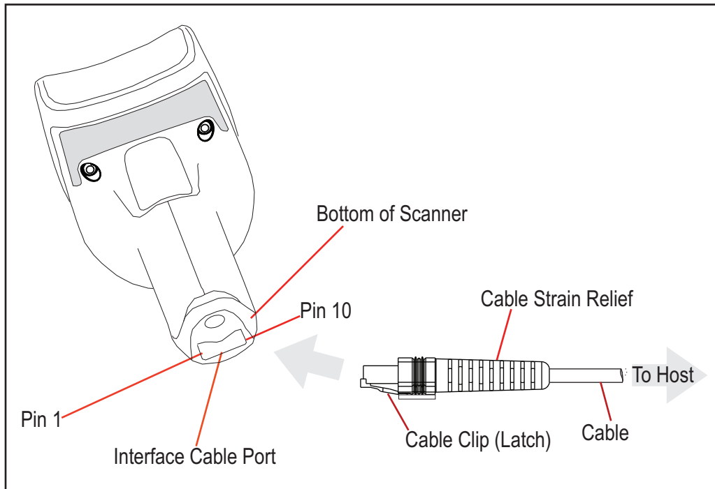
Figure 9. Standard Cable Pinouts: Handheld
