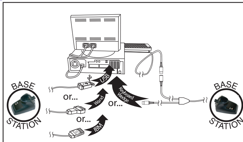
Figure 3. Connecting to the Host
