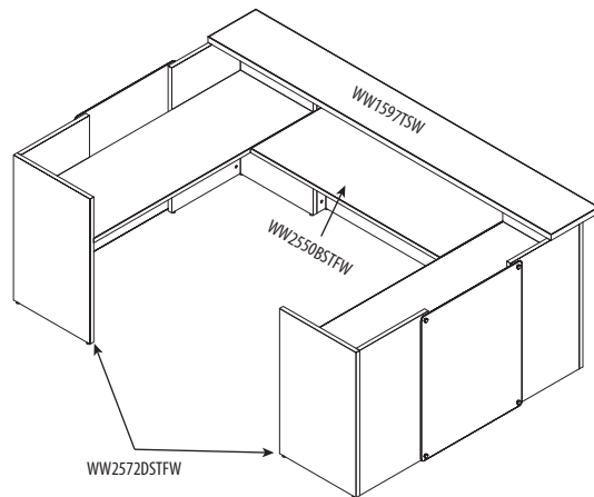
Fig. F - 2 Main Shells with Reception Bridge (Counter on reception bridge spanning main shells)
