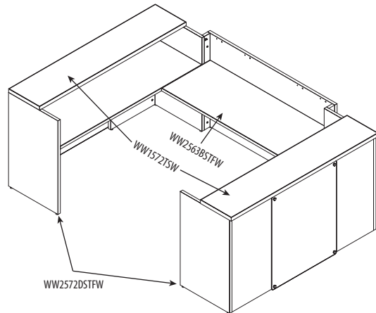
Fig. D - 2 Main Shells with Reception Bridge (Counters on main shell)
