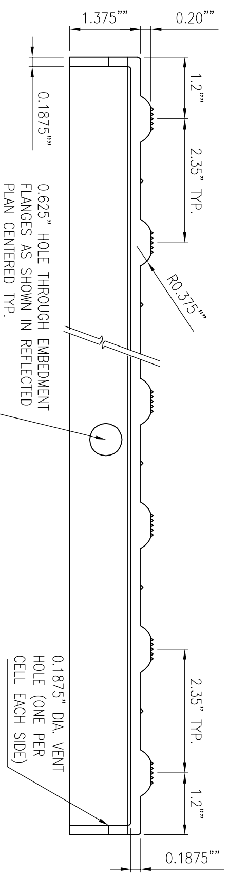
SECTION A-A (1/2 FULL)
