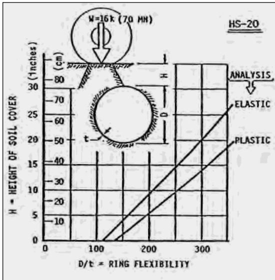
Figure 7. Minimum soil cover (with built-in safety factor) for pipes buried in compacted granular soil denser than 85% (ASTM D698 or AASHTO T-99) with wheel loads: W = 16 kips (70 MN) – HS-20 on unpaved surface
