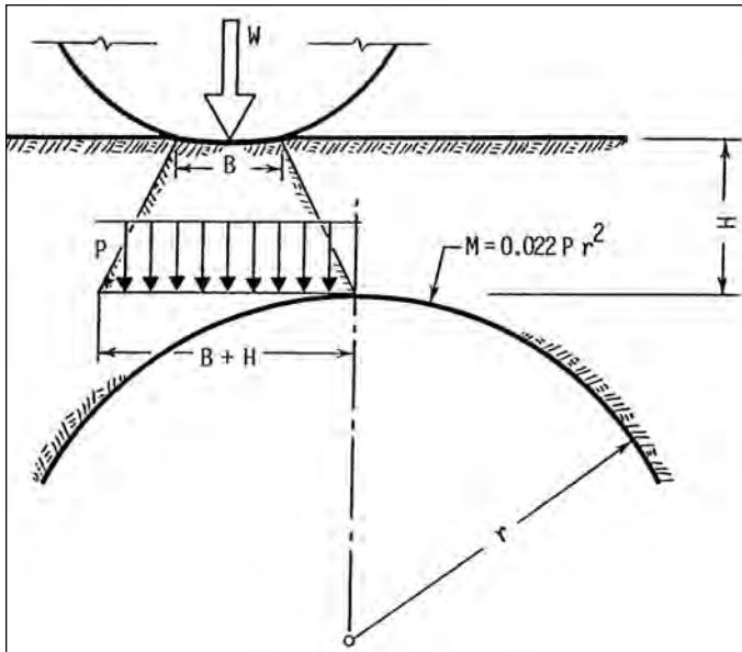
Figure 23. Conditions for inversion of the top of an unpressurized pipe due to a surface wheel load and a minimum cover, H, showing the truncated pyramid punched through to the pipe, and showing the maximum moment, M.
