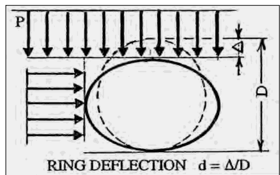
Ring deflection
