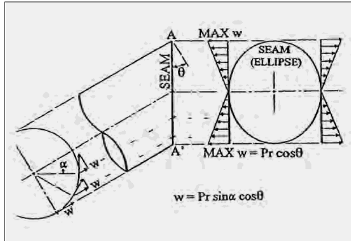
Figure 32. Force, w , on the mitre seam per unit length of circumference, due to internal pressure, P , where hoops are cut.
