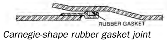
Rolled-groove rubber gasket joint
