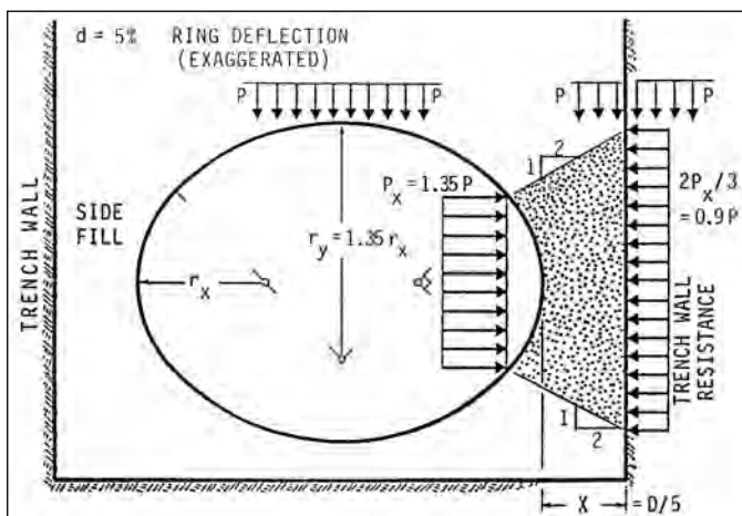
Figure 24. Trench wall support required for flexible stability, showing the sidefill wedge at soil slip. In this case, ring deflection is d = 5\% and width of sidefill is X = D/5 . In this worst-case example, and in general, the required trench wall resistance is less than pressure P on the pipe.
