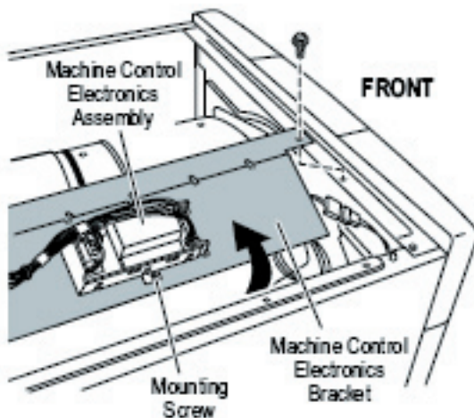
Figure 16. Remove machine control electronics from mounting bracket.
