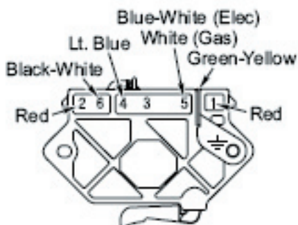
Pluggable Drive Motor Switch
