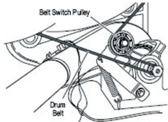
Figure 7. Carefully remove drum belt.
