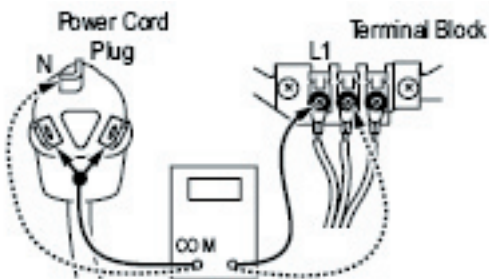
Figure 4. Plug-to-terminal connections for electric dryer.
