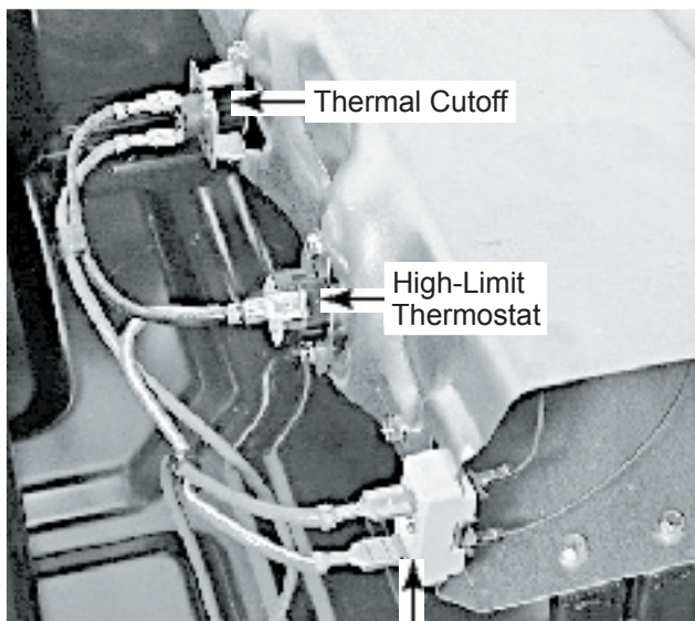
Heater Terminals
