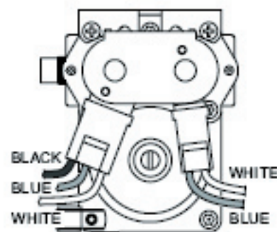
Gas Valve - Gas Dryer
