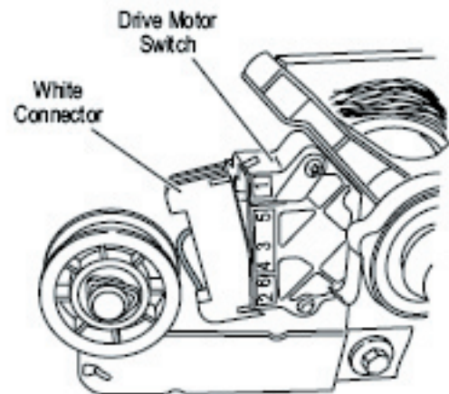
Figure 8. Remove white connector.
