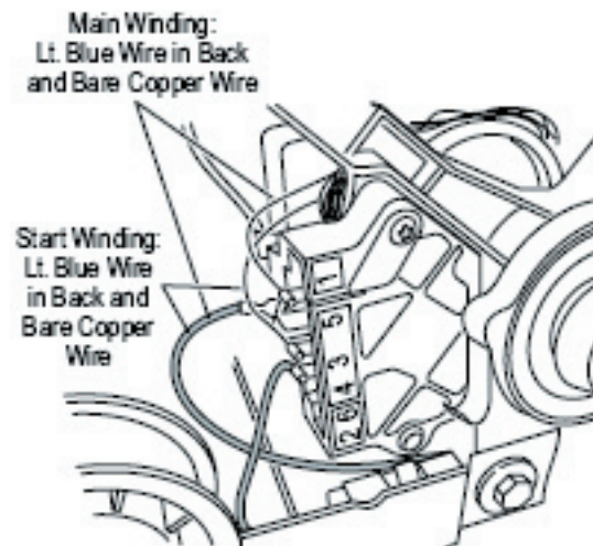
Figure 9. Main and start winding measure points.
