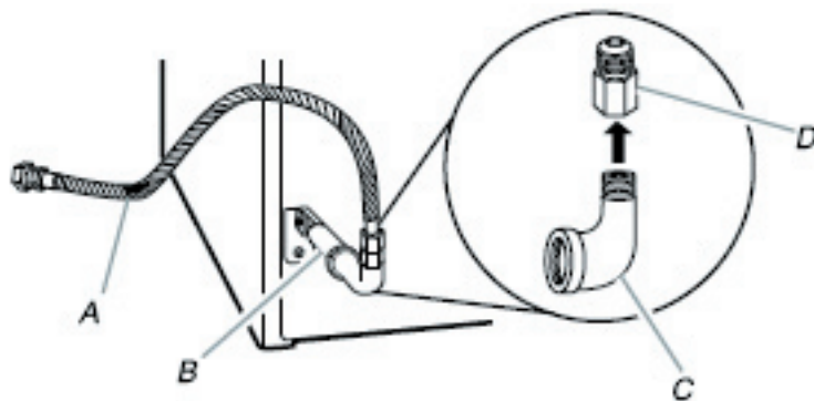
A. 3/8" flexible gas connector B. 3/8" dryer pipe C. 3/8" to 1/2" pipe elbow D. 3/8" pipe-to-flare adapter fitting
