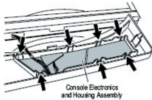
Figure 19. Locate seven locking tabs.
