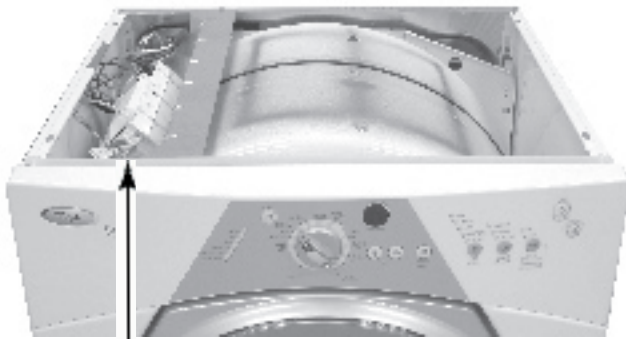
Machine Control Electronics Assembly
