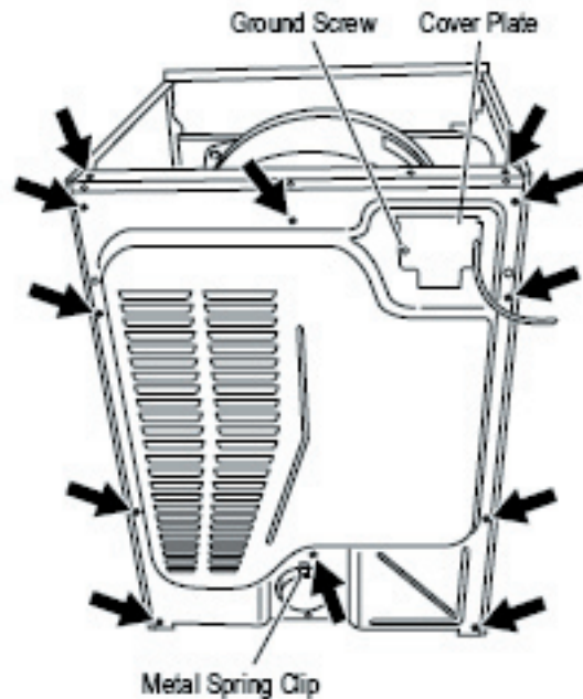
Figure 20. Remove 12 screws.
