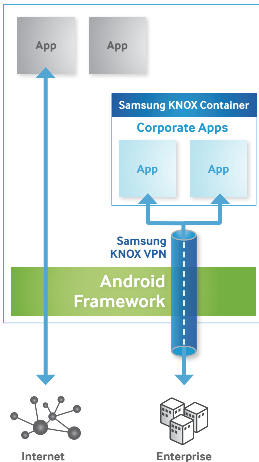
Figure 6 – Per-App VPN in Samsung KNOX
