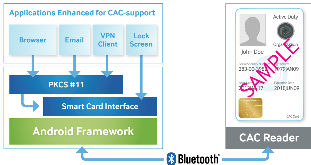
Figure 9 – Samsung KNOX Support for CAC
