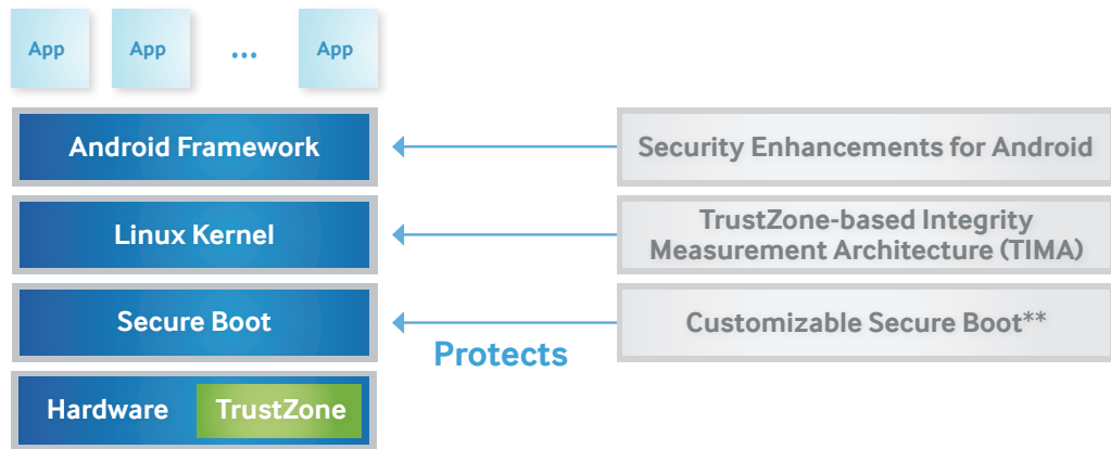
Figure 2 – Samsung KNOX System Security Overview
