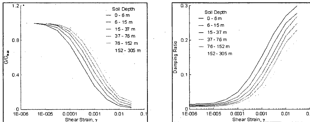
Figure 1 Example Graphs of Shear Modulus and Damping Ratio versus Strain (from EPRI, 1993)
