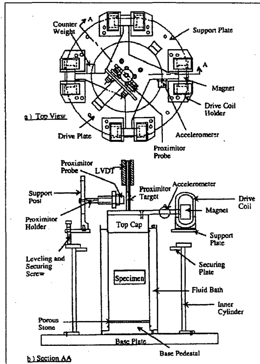
Figure 2 Schematic Drawing of Resonant Column/Torsional Shear Apparatus (from Ni, 1987)
