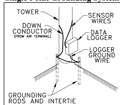
Figure 5.1 Single Point Grounding System
