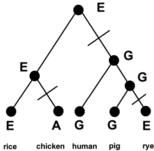
Figure 5.10: The tree after the top down pass. Mutations are now marked by a crossed branch. This tree contains three mutations at the column under consideration. Branches which are not marked have mutations at other columns.
